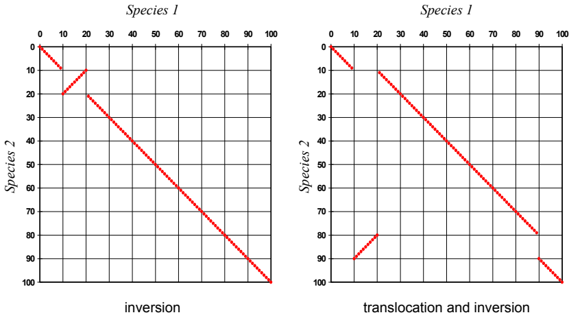
Figure 2. Hypothetical whole genome map dot plots. On the left is the pattern expected from two maps that differ only by a simple inversion. On the right is the plot for two maps that differ by a translocated inversion.
