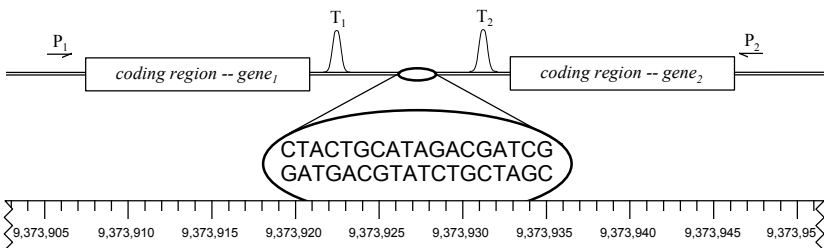
Figure 7. A simplistic view of the discrete coding-sequence model of the gene. Here, the fact that genes may be oriented in either direction in DNA is shown by reversing the placement of the promoter and terminator signals for the second gene. By this model, the locus of a gene corresponds to the address in base pairs of its start and stop signals.
