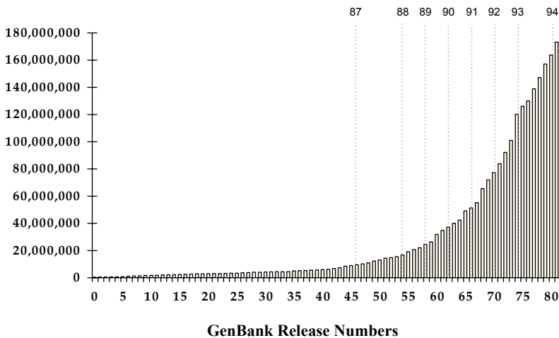
Figure 1. The growth of base pairs of sequence data in GenBank, 1 from Release 1 through Release 82. The year boundaries beginning with 1987 are given at the top of the figure. The
