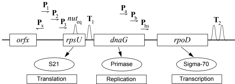
Figure 8. The MMS operon in E. coli contains a complex set of control and coding regions. Transcription of the rpoD coding region can begin from any of a half dozen promoters, some of which are embedded in the coding region of the dnaG gene. (Lupski, et al., 1989)
