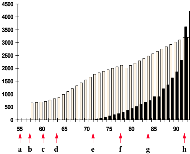
Figure 11. The increase in number of known enzymes (shaded bars) and known human genes (solid bars). The arrows indicate significant events in the history of enzyme nomenclature: a = Enzyme Commission formed, b = commission preliminary report, c = commission final report, d - h = appearance of five editions of Enzyme Nomenclature .
