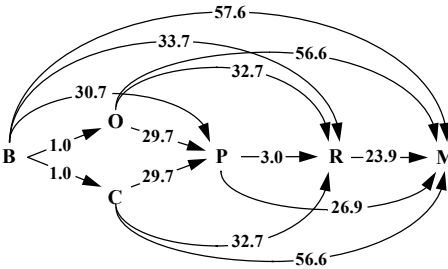
Figure 10. Data structures for genetic maps reflect the underlying conceptual models for the maps. Many geneticists still think of maps as ordered lists, and ordered list representations are used in many genome databases. Directed acyclic graph (DAG) data structures can be represented pictorially (left) or tabularly (right). Depending on their use, DAGs may be represented as transitive reductions or transitive closures.
