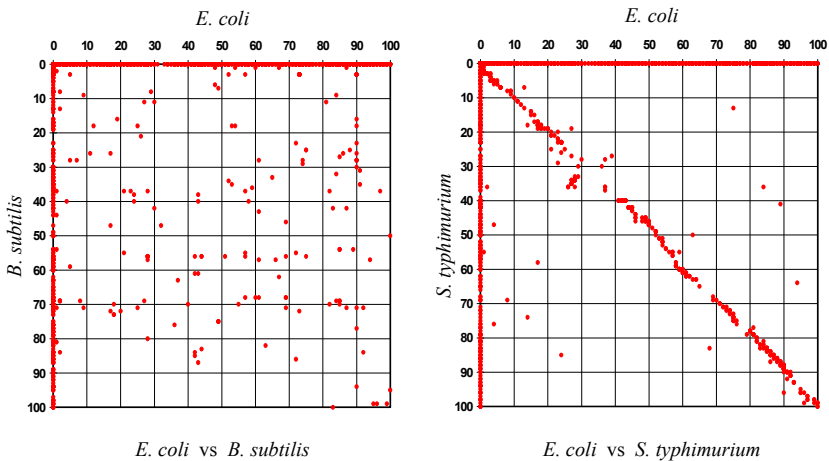
Figure 3. Whole genome map dot plots show essentially random distributions of homologous genes when the maps of E. coli and B. subtilis are compared. However, a similar plot of E. coli and S. typhimurium shows an obvious diagonal and gives some evidence of the well known inversion in the 30-40 minute region (Sanderson and Hall, 1970; Riley and Krawiec, 1987). Individual outliers may indicate small rearrangements or simply errors in the data. (Homology data from Abel and Cedergren, 1990.)
