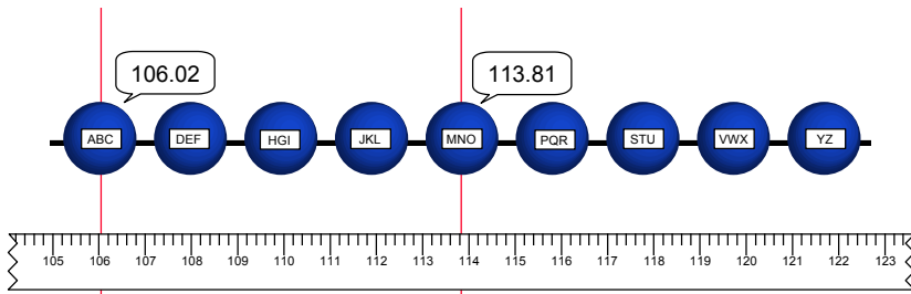
Figure 6. According to the “beads on a string” model of genes, mapping just involved determining the correct order of the beads and the correct address, or locus, for each bead.
