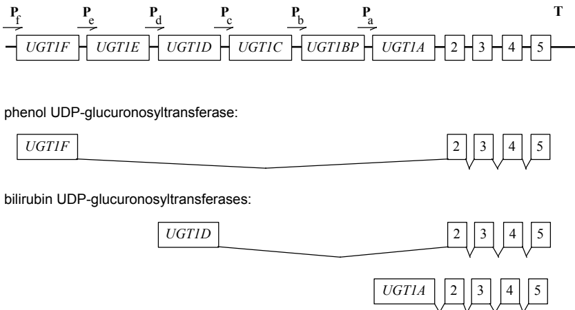
Figure 9. The UGT1 locus in humans is actually a nested gene family that yields multiple transcripts through alternative promotion. Each promoter produces a transcript that is spliced so that the exon immediately adjacent to the promoter is joined with the four terminal exons shared by all of the transcripts. (Ritter, et al., 1992)
